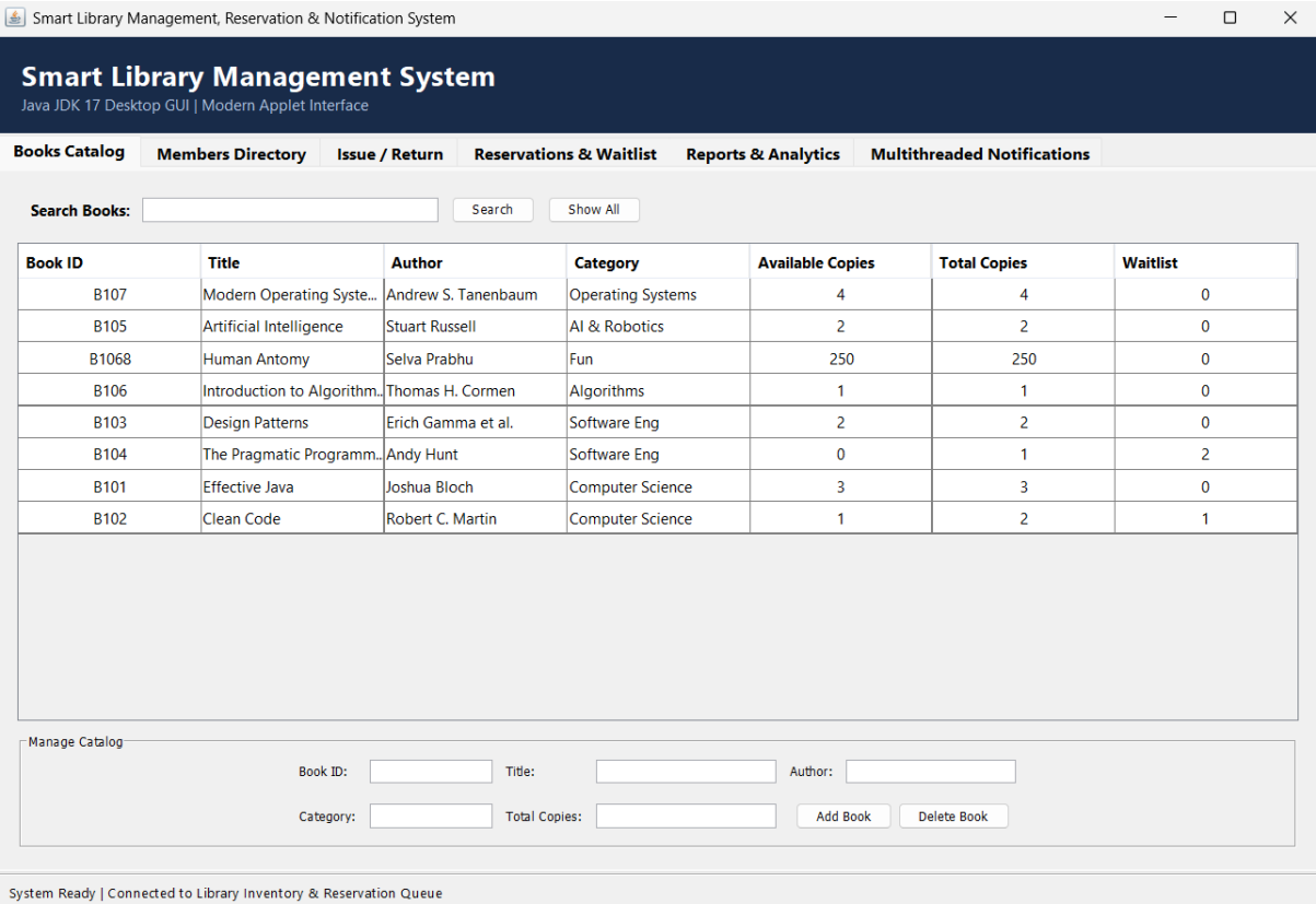
Figure 2: Add Book
